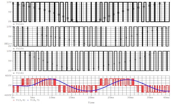
b). SPWM switching control method
