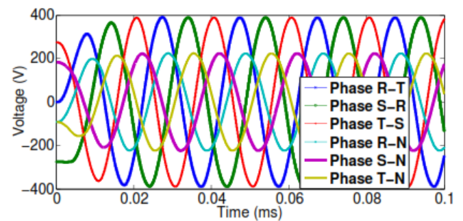
(c). LCL 2-leg
