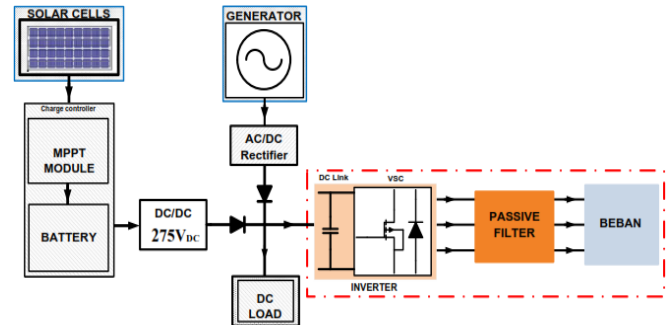
Fig. 1. Diagram of a hybrid grid and solar-based power generation system with DC power source coupling.
