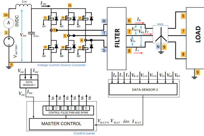
Fig. 2. Inverter system models.
