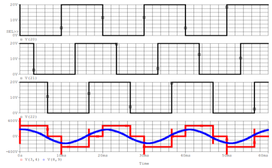
a). PWM switching control method
